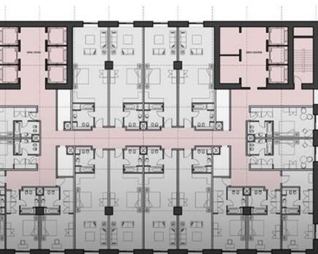
HOTEL TYPICAL FLOOR-TYPE II
