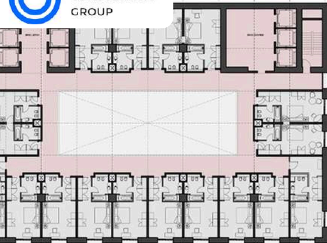
HOTEL TYPICAL FLOOR-TYPE I
